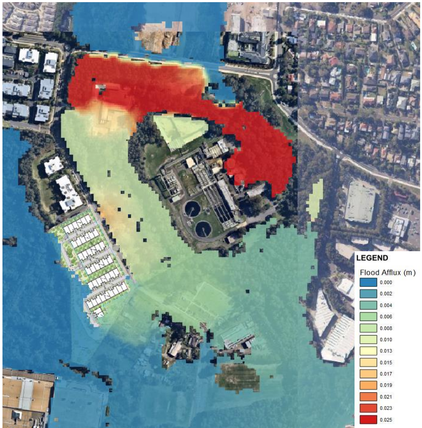
Figure 14 – 1% AEP 1440min Narrabeen Afflux
