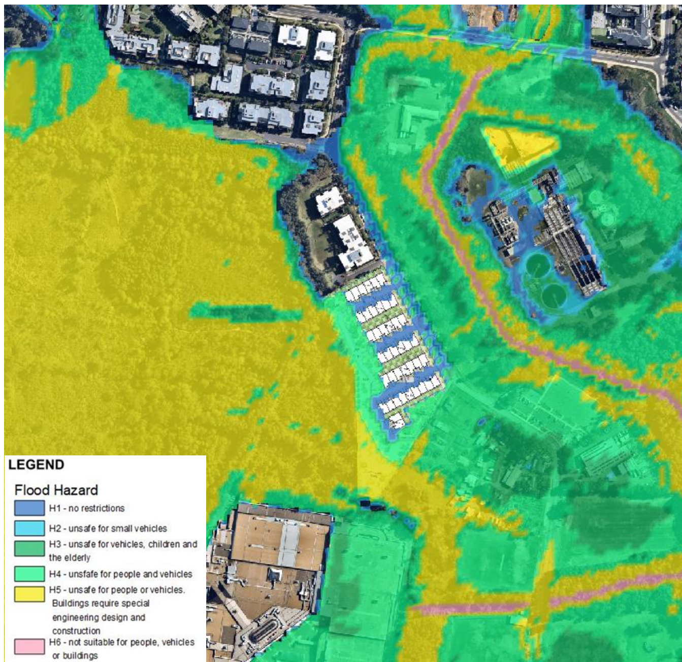
Figure 35 – PMF Storm at 180 mins
