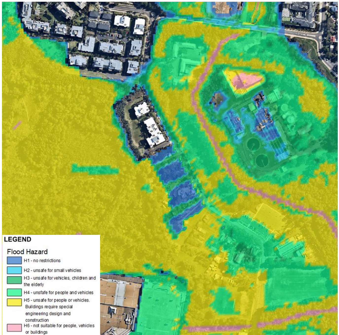
Figure 37 – PMF Storm at 210 mins
