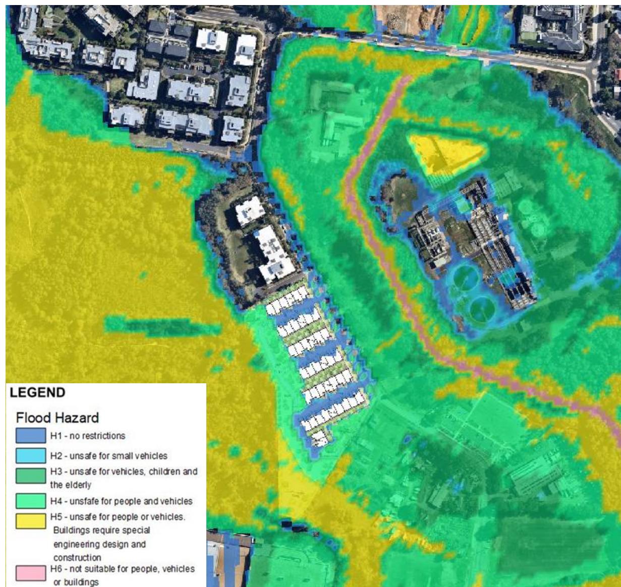
Figure 42 – PMF Storm at 10 hours 30 mins
