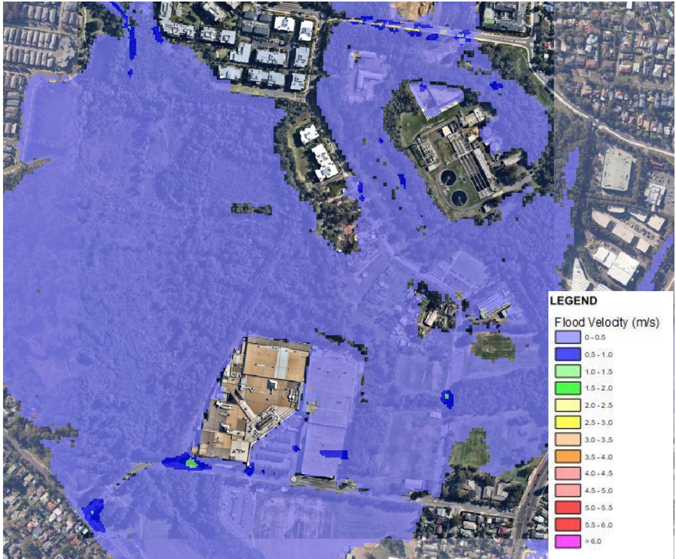
Figure 17 – 1% AEP 1440min Existing Velocities
