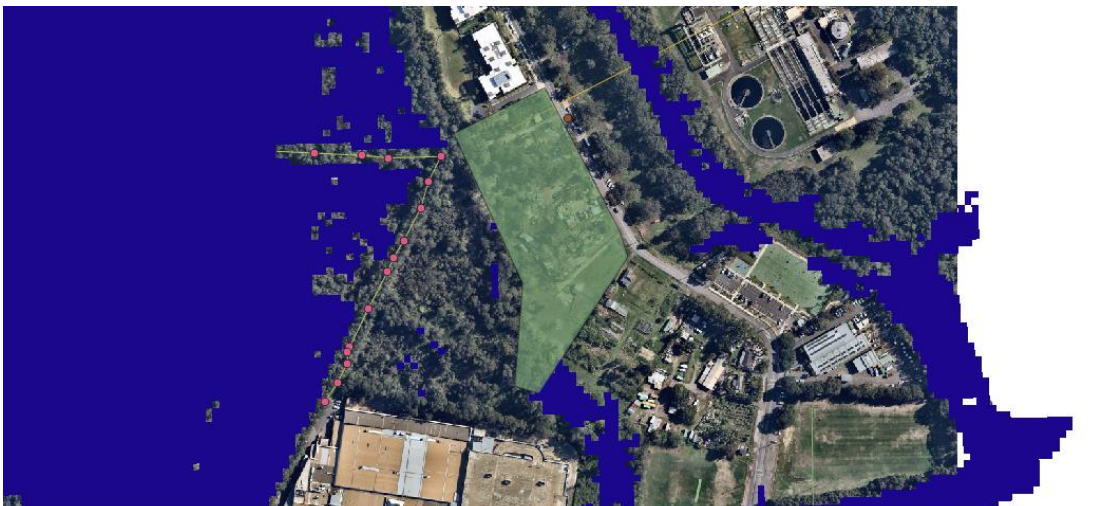
Figure 7 – 1% AEP Storm at 8 hours
