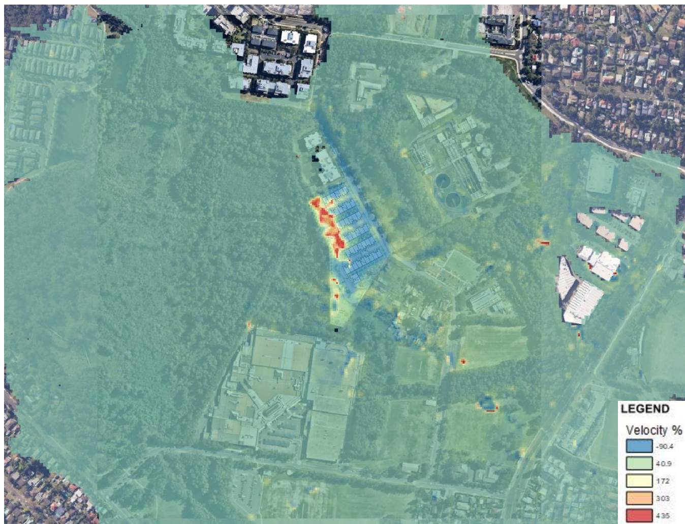
Figure 23 – PMF 360min Velocity % Afflux
