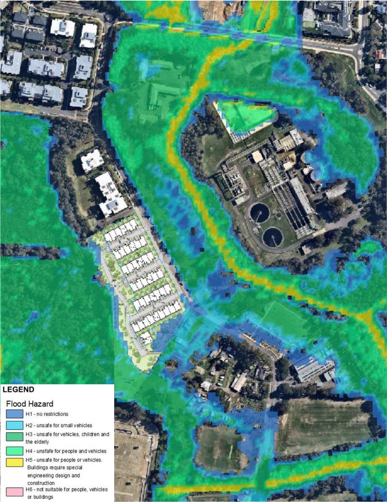
Figure 33 – PMF Storm at 75mins
