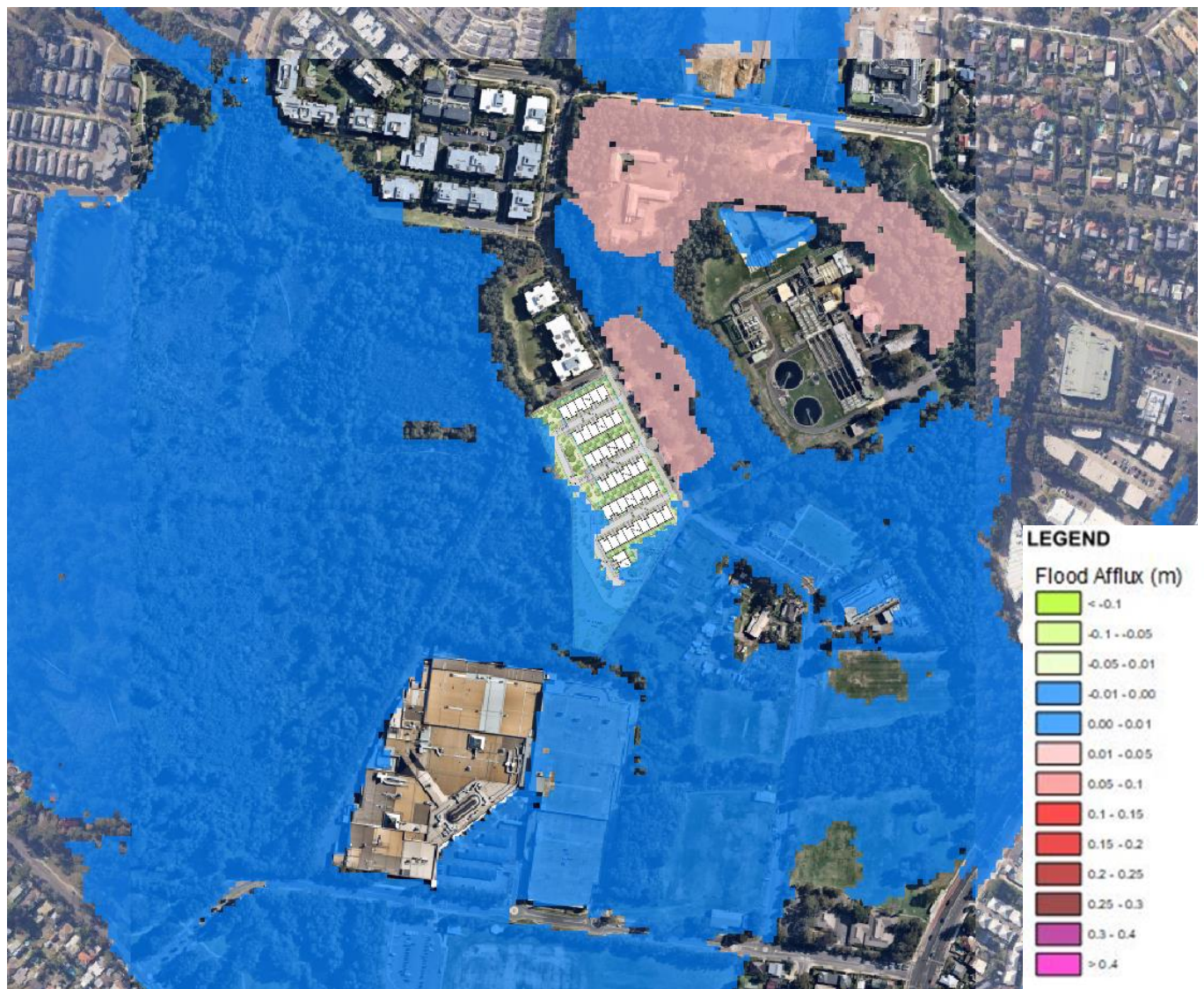
Figure 13 – 1% AEP 1440min Afflux
