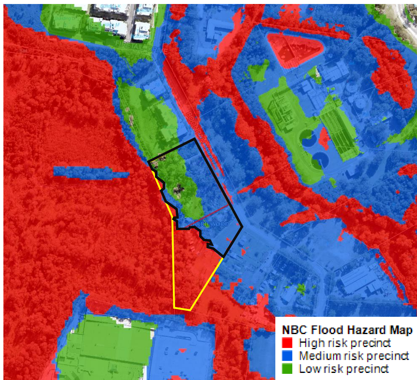
Figure 26 – Flood Risk Precinct Map
