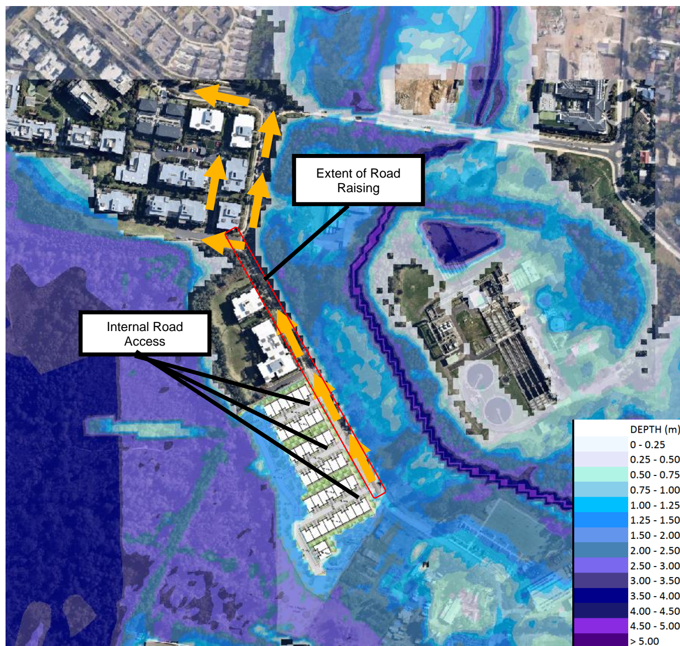
Figure 31 – Flood Evacuation Route in the 1% AEP + CC
