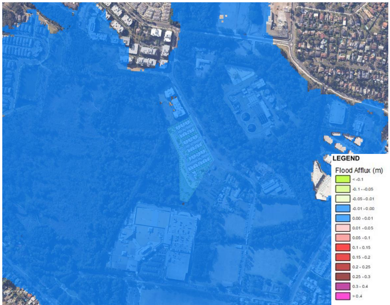
Figure 21 – PMF 360min Afflux
