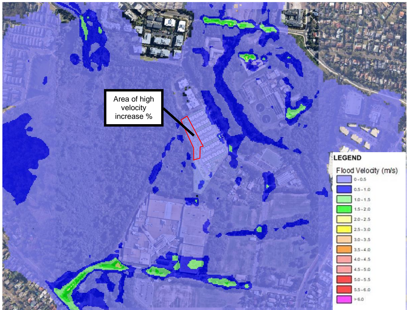
Figure 25 – PMF 360min Developed Velocities
