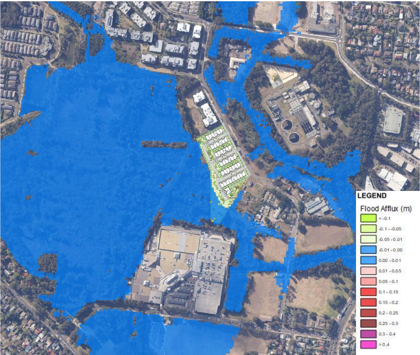
Figure 11 – 50% AEP 1440min Afflux
