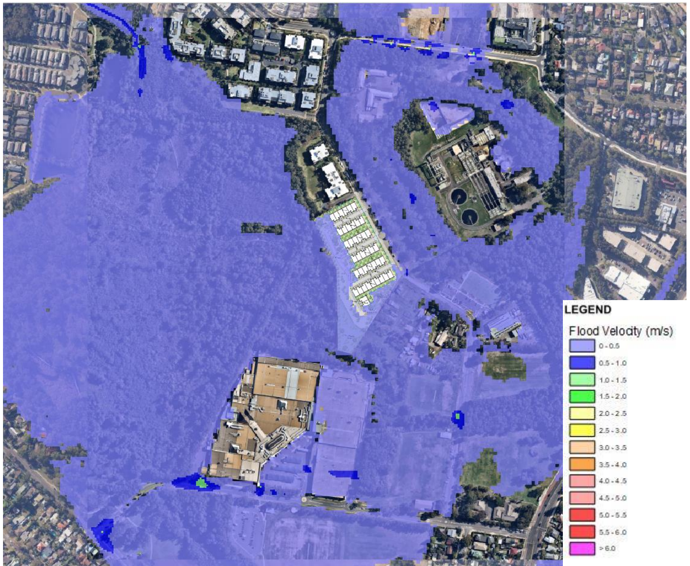
Figure 18 – 1% AEP 1440min Developed Velocities
