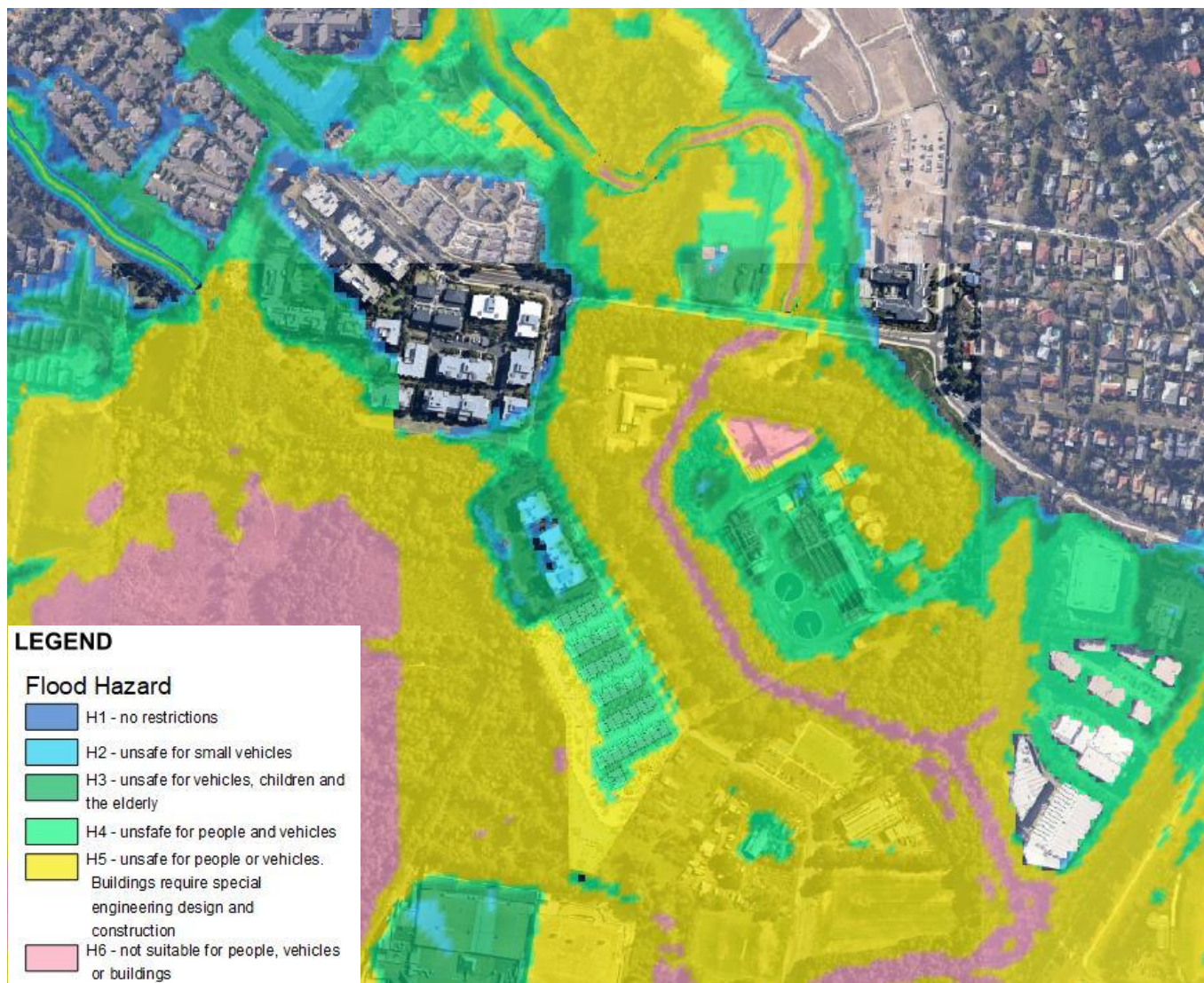
Figure 30 – PMF 360min Developed ZAEM1 Hazard Rating
