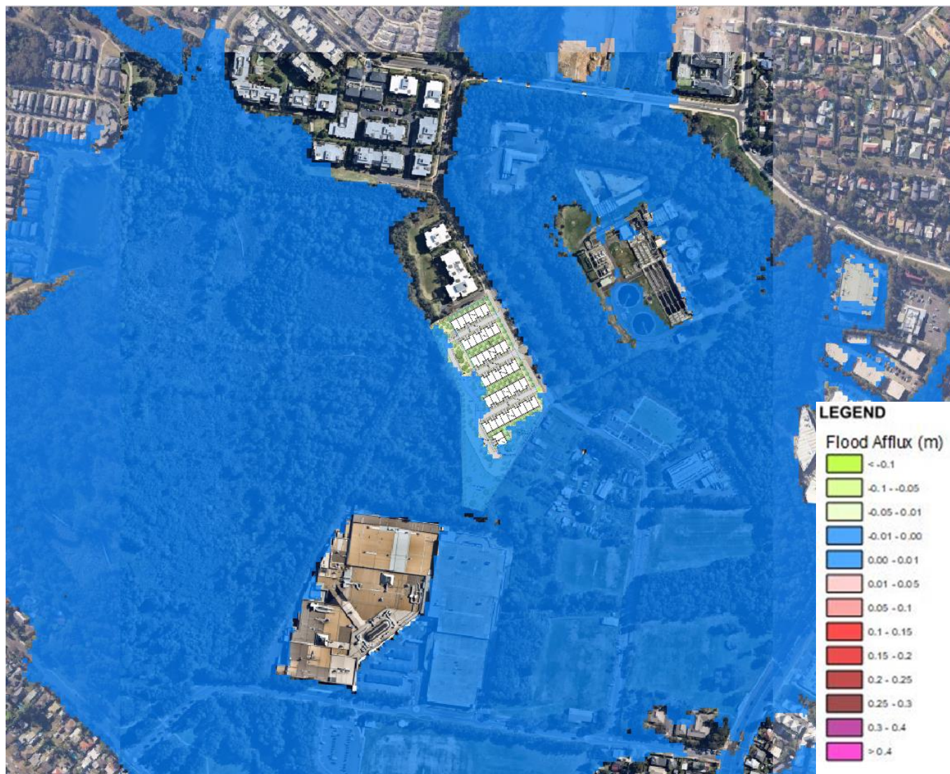
Figure 16 – 1% AEP 540min + CC Afflux
