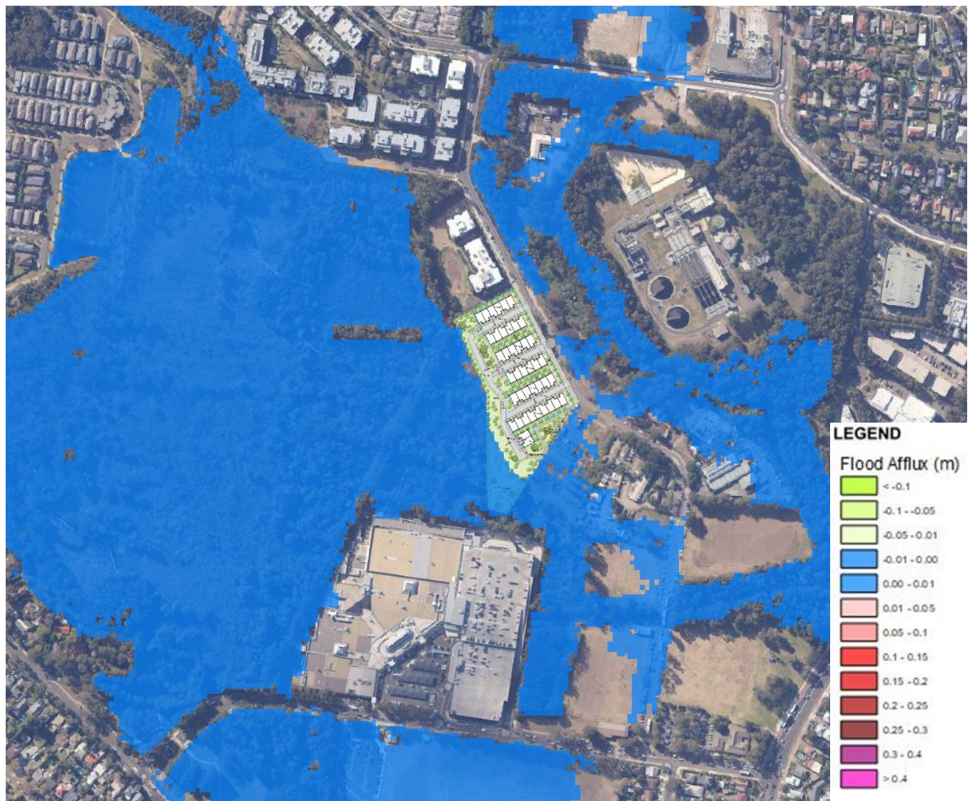
Figure 12 – 20% AEP 1440min Afflux
