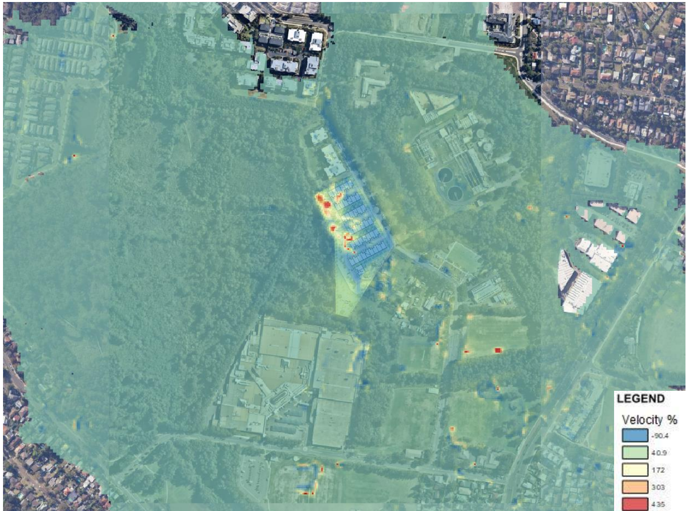
Figure 24 – PMF 360min + CC Velocity % Afflux
